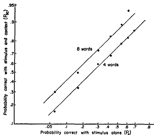
FIG. 6. The same data as in Figure 5; plotted as \logit P_{sc} = K + \logit P_s . (The lines are fitted by eye with the predicted slope of unity.)
